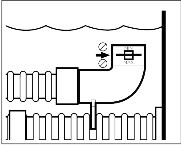
5 Inspect Flow Gauge and Adjust as Required
